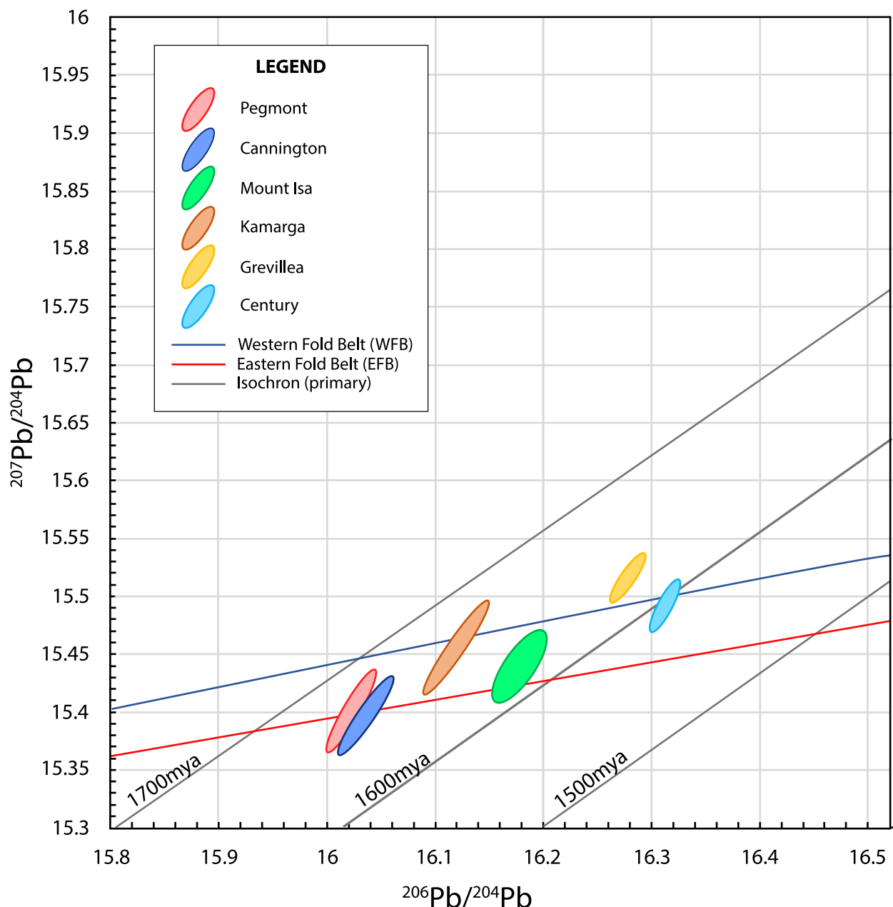
Figure 3.2. Conventional Pb isotope plot with regional growth curves and primary isochrons showing containment ellipses for samples of main-stage sulfide of Mount Isa region base metal ore deposits and significant prospects (from the database and graphs of Carr et al., 2001).
