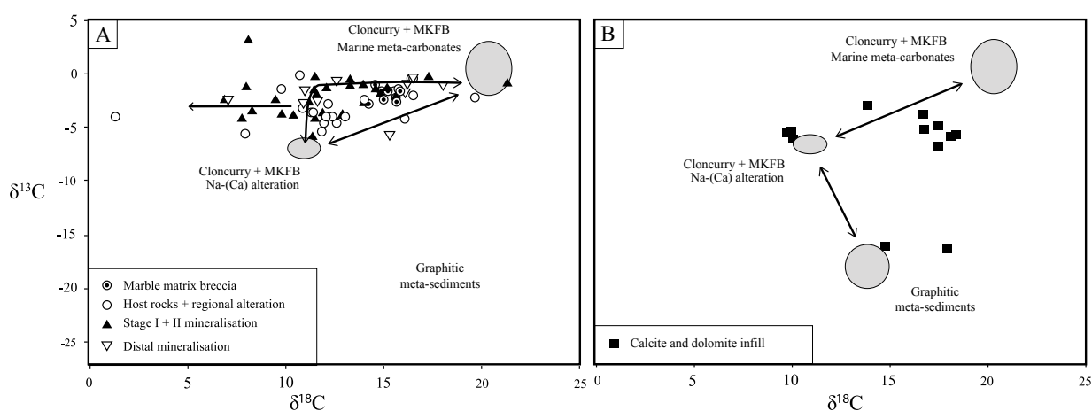
Figure 4.8. \delta^{13}\text{C} vs. \delta^{18}\text{O} plots for carbonate from the Ernest Henry deposit and environs (A), and the Great Australia Cu deposit (B); arrows refer to data trends, not model trends; 'MKFB' is the exposed part of the Mary Kathleen structural domain (also known as Wonga Subprovince) (from Marshall et al., 2006).
