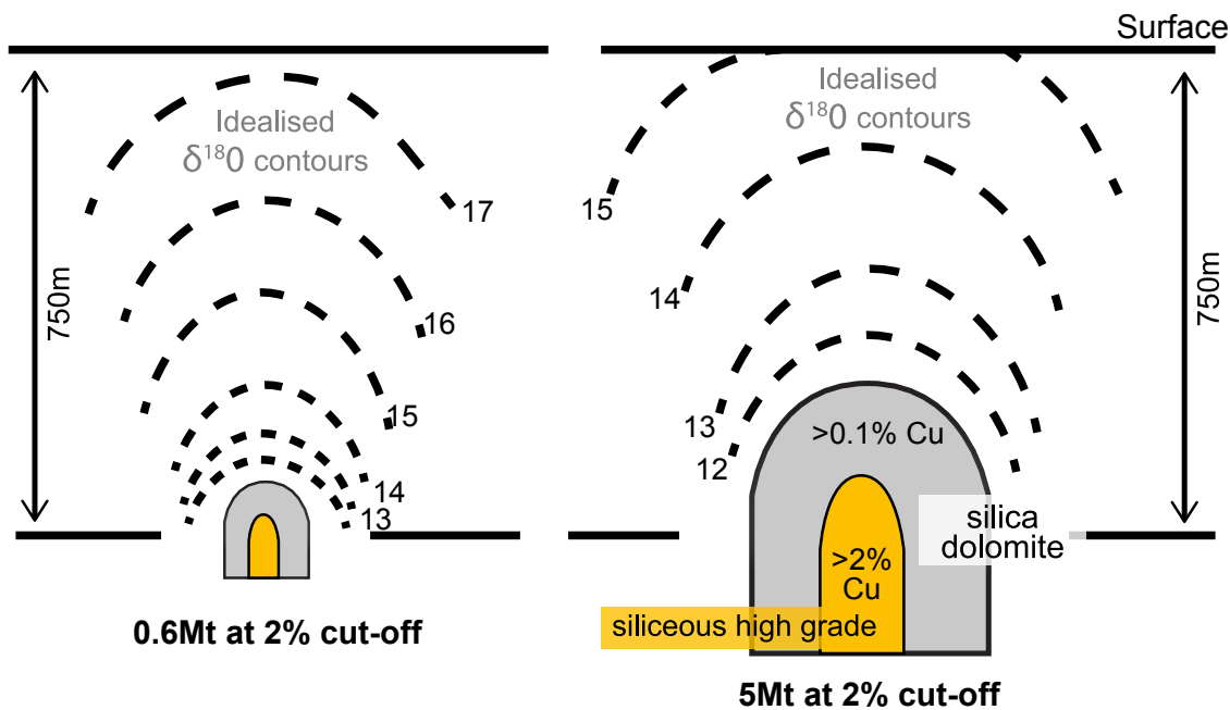
Figure 4.4. Cross sectional view of scaled and idealised \delta^{18}\text{O} contours above two Mount Isa-style Cu orebodies (from Hannan, 1991).
