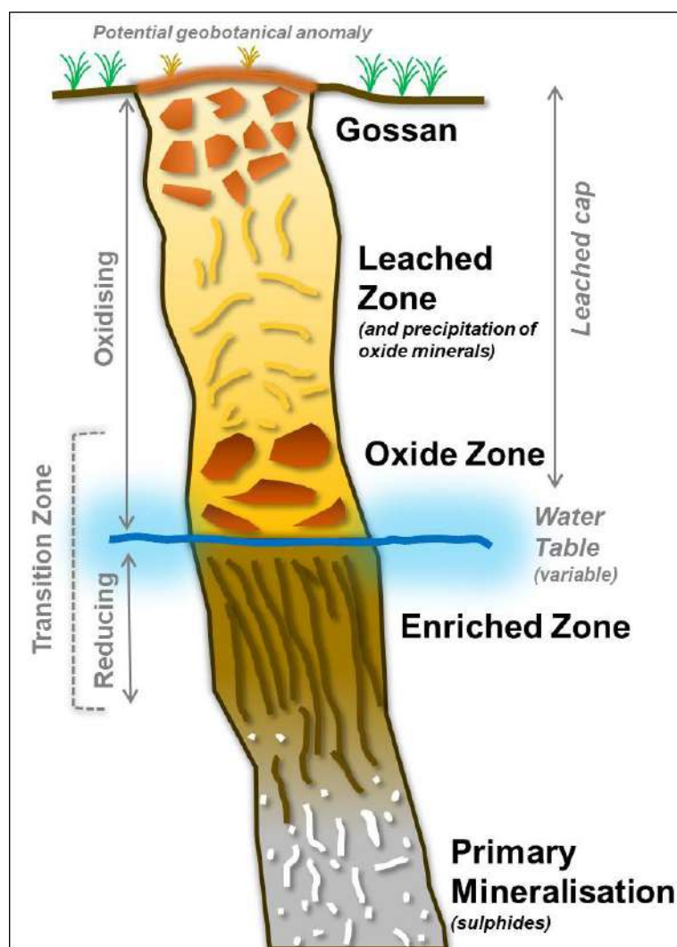
Figure 2.1. Schematic and idealised cross section of the internal structure of a gossan profile (after Taylor, 2016; Butt et al. , 2005, Scott et al. , 2002).
