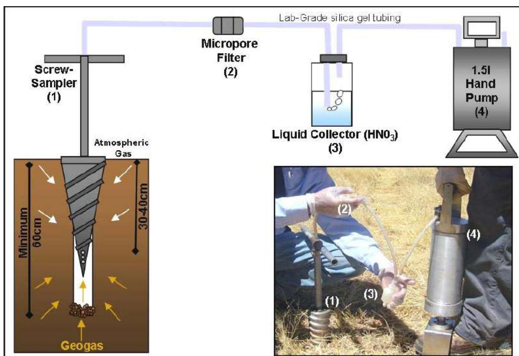
Figure 30, Simplified schematic for MSG collection process used in GTC project (after Wang et al, 2008). Inset picture illustrates sample collection in the field with numbers correlating to main diagram
