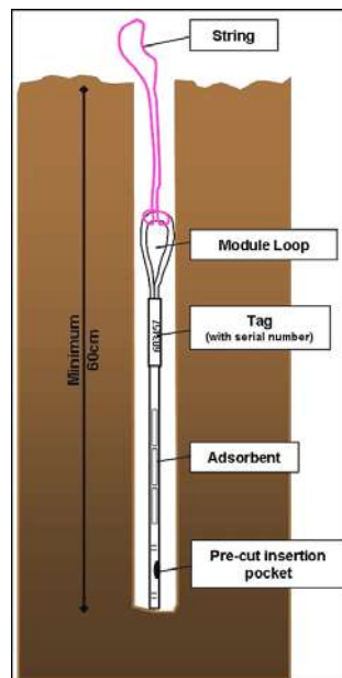
Figure 28, key components of the GORE module
