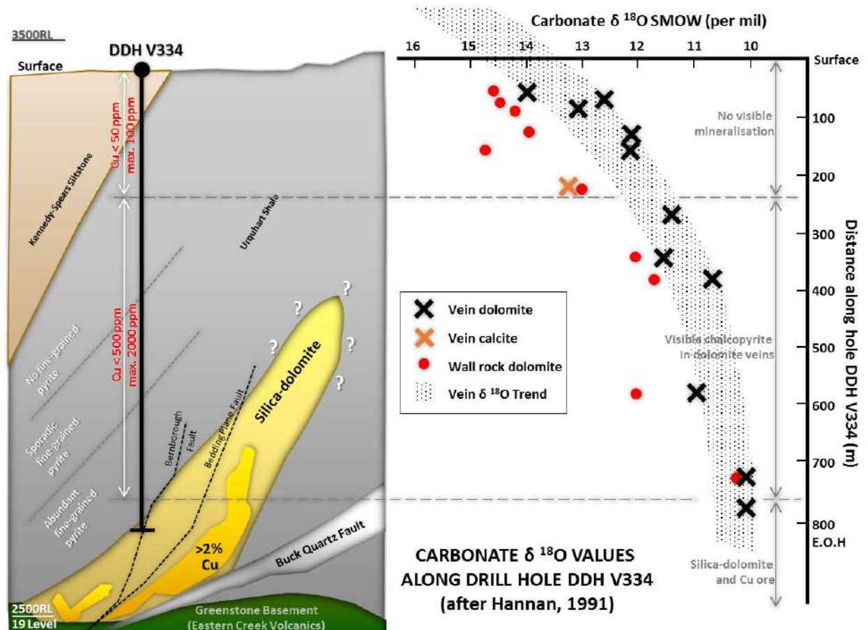
Figure 4.3. Left: cross section of Mount Isa Mine at 3340 mN with trace of drillhole V334 and simplified geology; right: carbonate (dolomite) O isotopic composition versus depth for DDH V334. (from Hannan, 1991)
