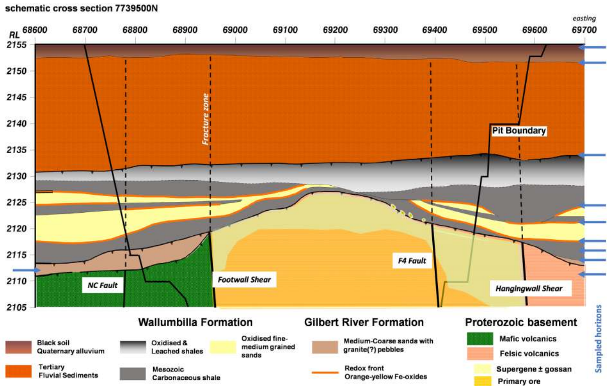
Figure 6.3. Cross section of the northern end of the Ernest Henry deposit, where paleotopographic relief is greatest and cover thickness the least (adaptation of figure 4 in Sheppard, 2001).
