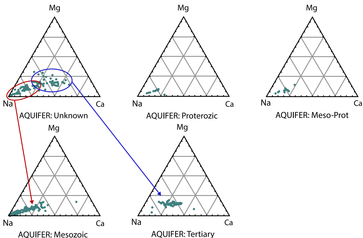
Figure 8.4. Mg-Ca-Na ternary diagrams for various aquifers (after Hannan & Sheppard, 2002).
