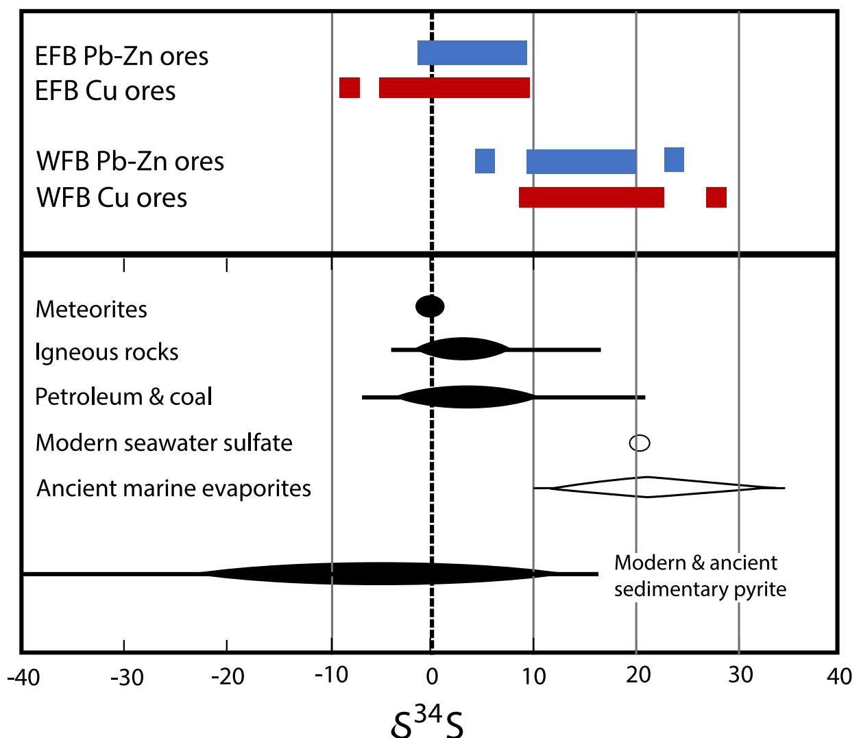
Figure 4.9. \delta^{34}\text{S}_{\text{CDT}} distributions of Mount Isa Inlier ore sulfides compared to global sulfur reservoirs; red bars apply to chalcopyrite and blue bars to galena \pm sphalerite (sources—Seal II, 2006; Davidson & Dixon, 1992; Case, 2016; Painter et al. , 1999).
