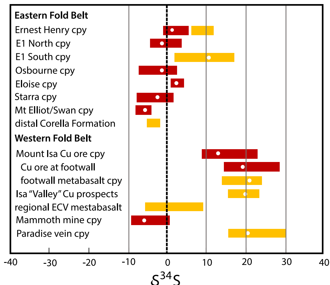
Figure 4.10. Ranges and medians of \delta^{34}\text{S}_{\text{CDT}} values for chalcopyrite in Mount Isa Inlier copper \pm gold deposits (red bars) and prospects (yellow bars). (sources—Case, 2016; Davidson & Dixon, 1992; Hannan et al. , 1993; Painter et al. , 1999).
