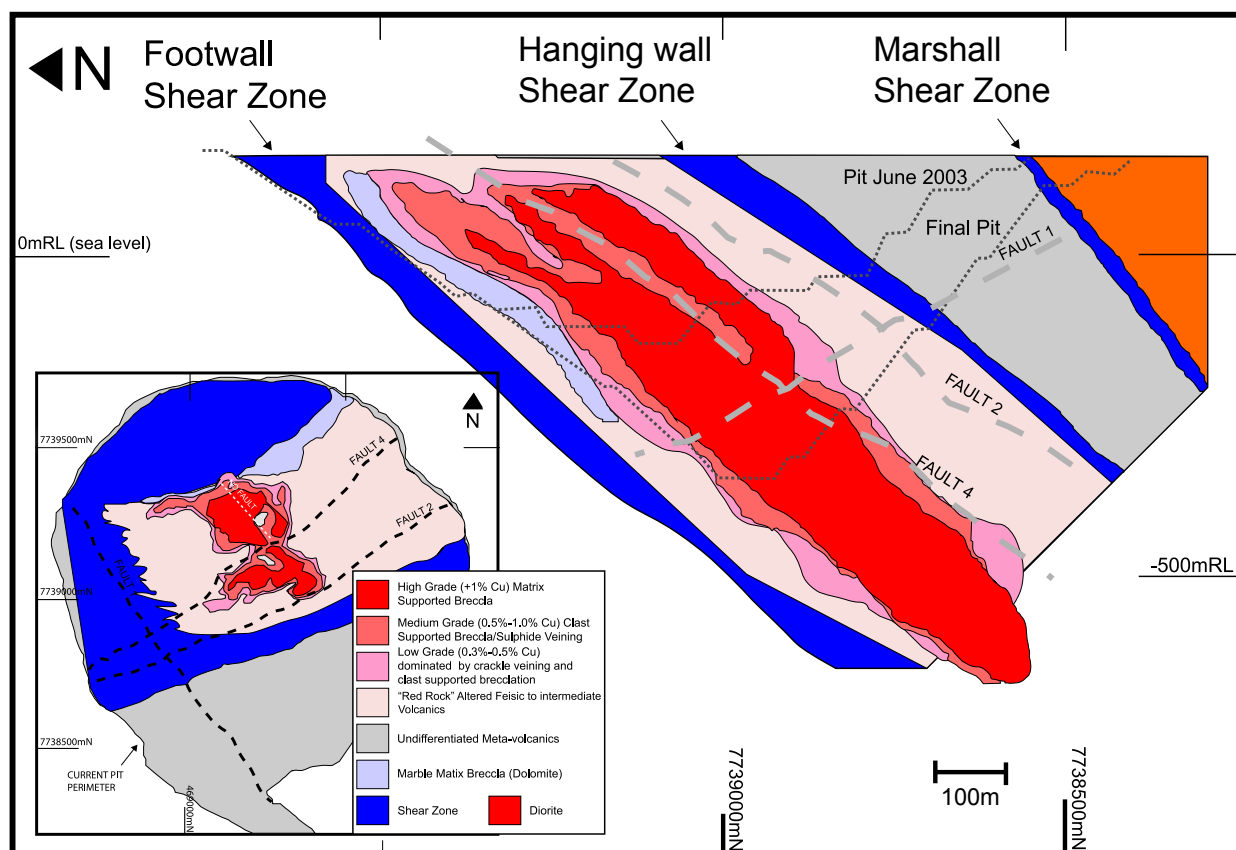
Figure 6.2. Geology and Cu-grade distributions of the Ernest Henry Cu-Au deposit—long section (upper frame), plan view (left frame, unknown RL) and legend (from Lilly et al., 2017).
