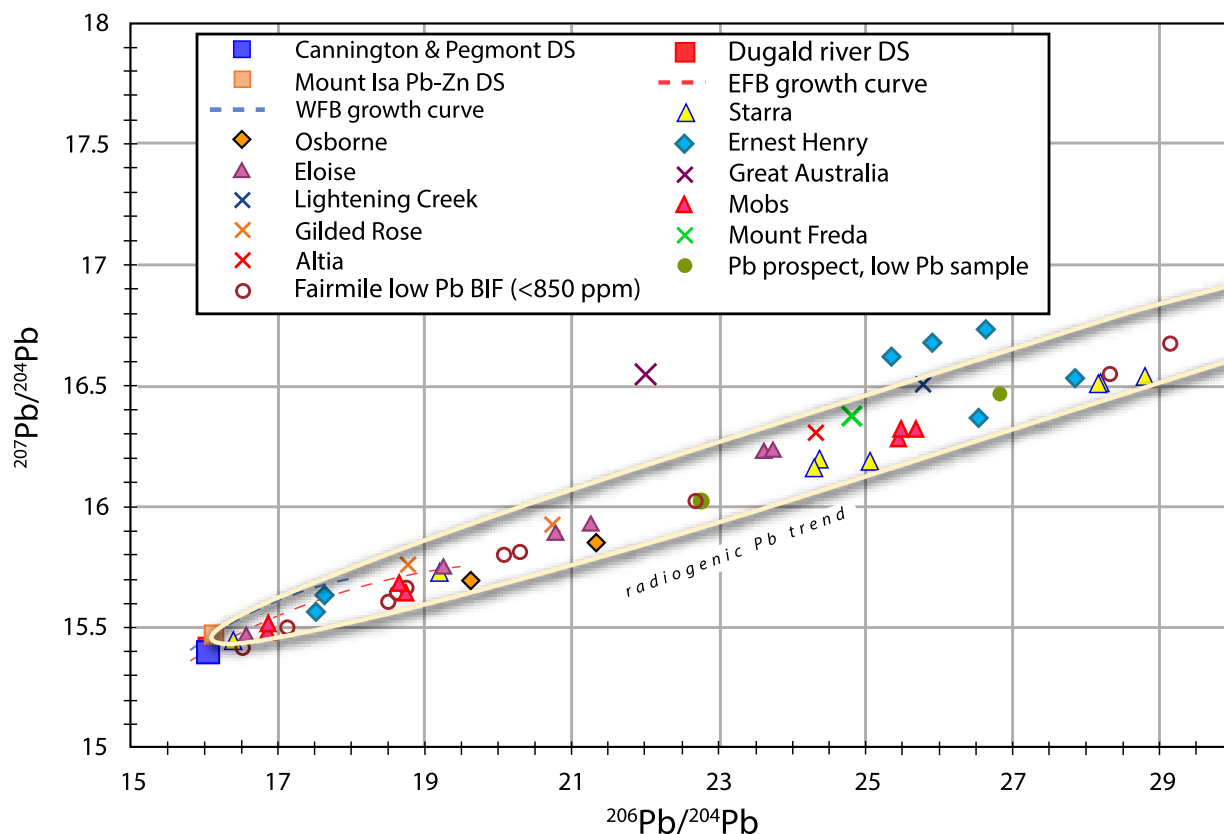
Figure 3.9. Conventional Pb isotope ratio plot of Eastern Fold Belt IOCG deposits and prospect samples in relation to a 95% enclosure ellipse referred to as the radiogenic Pb trend (which extends off-scale to ^{206}\text{Pb}/^{204}\text{Pb} values of 100 or more).
