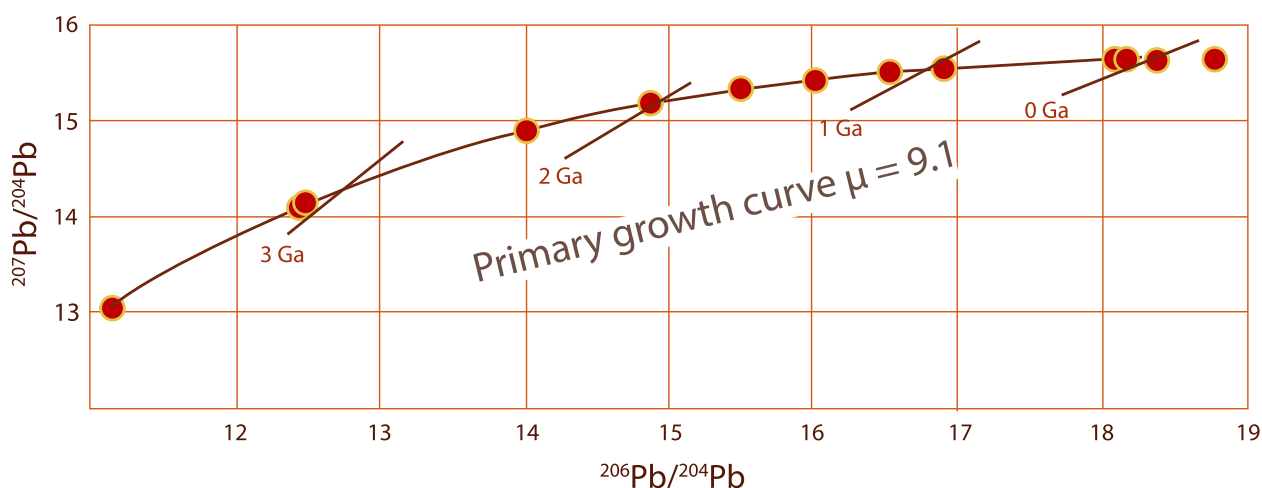
Figure 3.1. Pb isotope data for stratabound ore deposits (from data in Albarede & Juteau, 1984).
