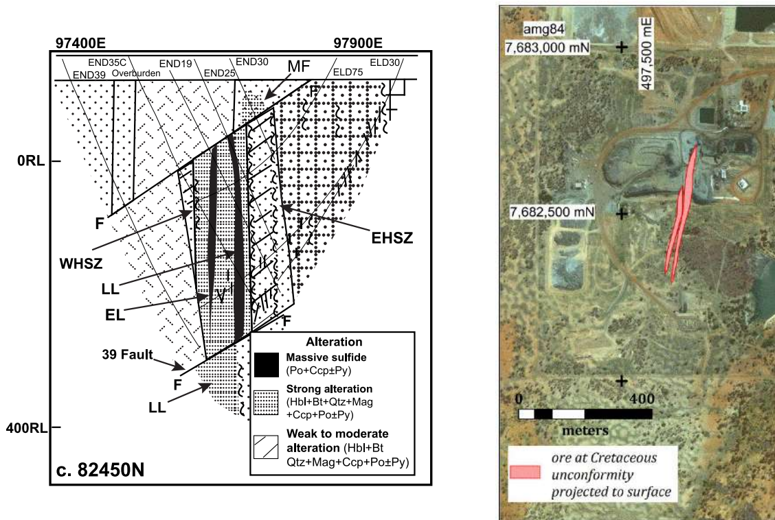
Figure 6.27. Geologic cross section of the Eloise deposit (left) and map of projected ore limits on aerial image of mine infrastructure at 2009 (from Baker, 1998, and Lilly et al. 2010, respectively, modified).
