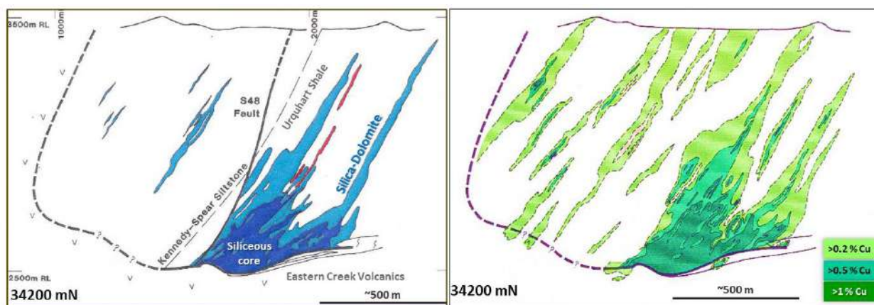
Figure 4.5. Summarised distributions of silica-dolomite (left) and copper grades (right) for a composite section of Mount Isa Mine centred at 34200 mN (from Hannan et al. , 1991).
