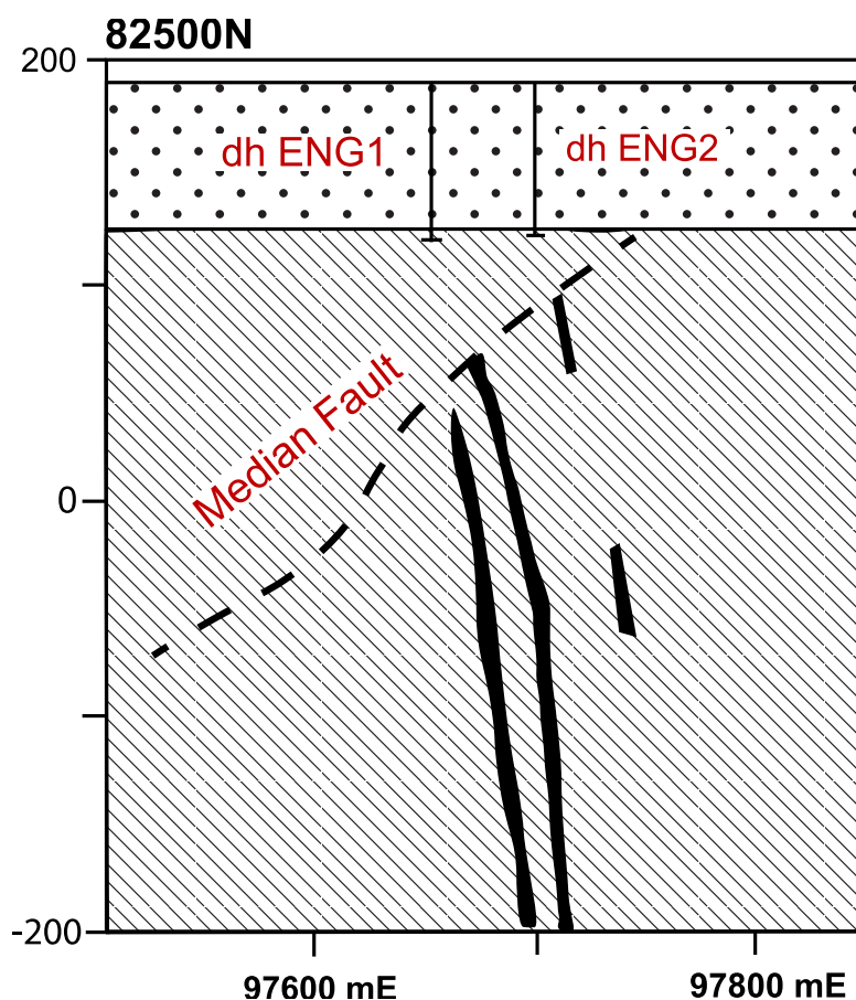
Figure 6.33. Cross section of Eloise deposit at 82500 mN with simplified geology and analysed lengths of drill holes in Mesozoic mudstone cover (from Li Shu & Robertson, 1997, modified).
