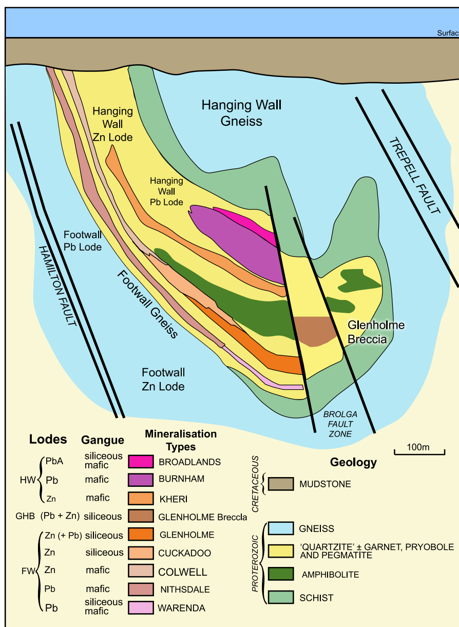
Figure 6.40. Simplified geologic cross section of the Cannington deposit (from Readford & Curypko, 2017).
