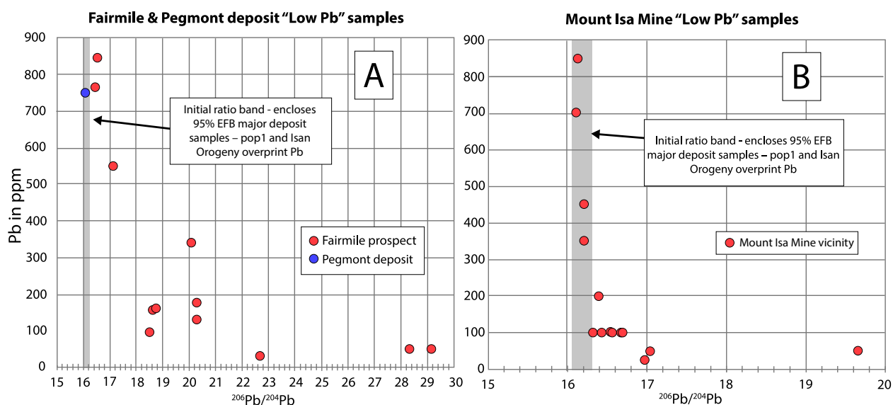
Figure 3.8. Pb content versus Pb isotopic composition plot of samples classified as ‘low Pb’ from Fairmile and Pegmont (A) and the vicinity of Mount Isa Mine (B).
