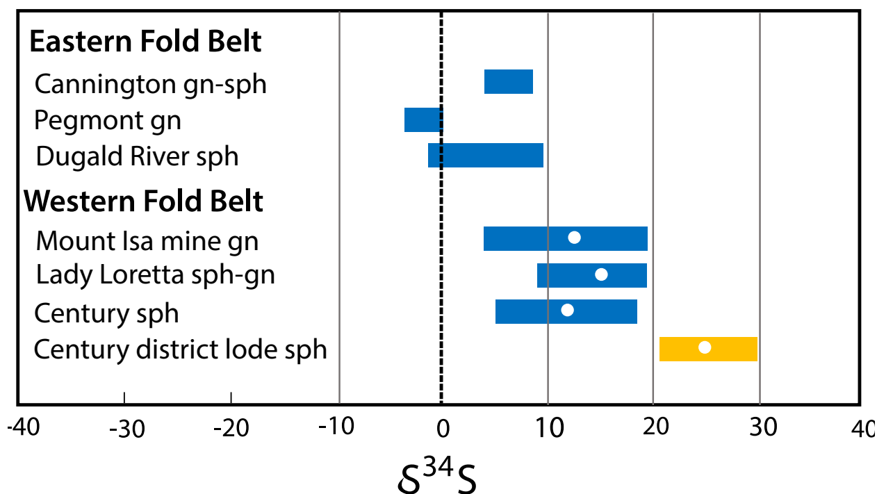
Figure 4.11. Ranges and medians of \delta^{34}S_{\text{CDT}} values for galena and/or sphalerite in Mount Isa Inlier Pb-Zn-Ag deposits (blue bars) and prospects (yellow bars) (sources—Davidson & Dixon, 1992; Broadbent et al. , 1998; Painter et al. , 1999; Walters et al. , 2002).
