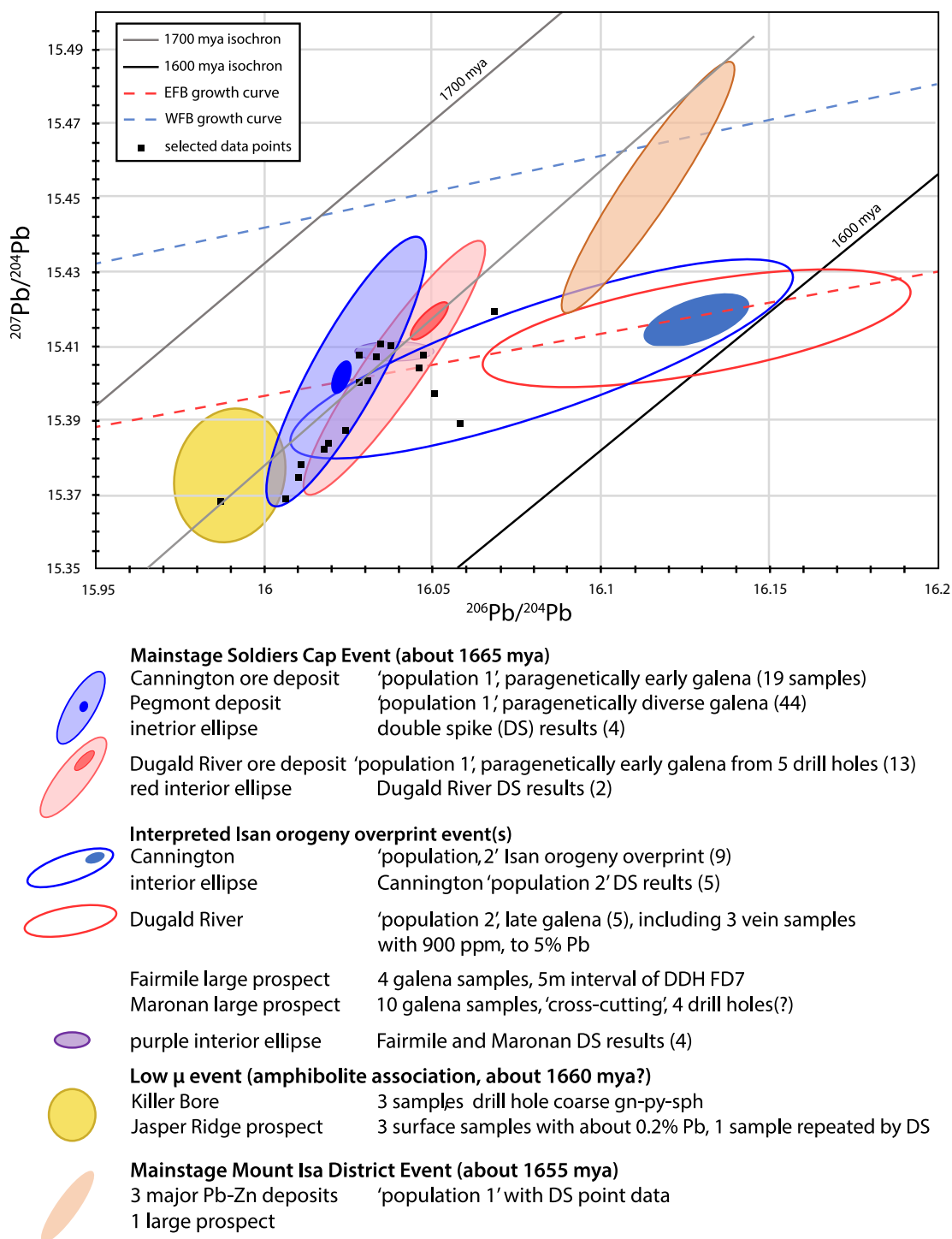
Figure 3.3. Conventional Pb isotope distributions, as 95% contain ellipses, of major Eastern Fold Belt Pb-rich deposits; showing main stage and orogenic overprint populations, fields of double spike data and other detail discussed in the text.
