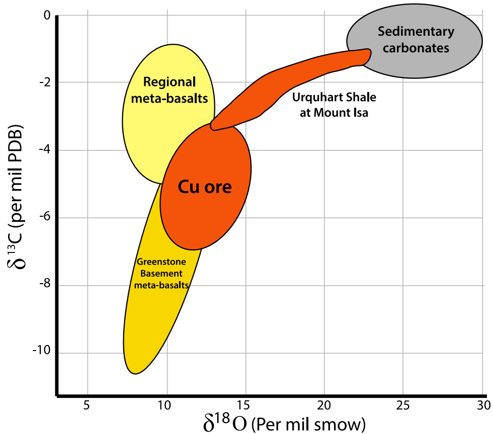
Figure 4.2. Summary of O and C isotopic compositions of carbonate in Urquhart Shale and Eastern Creek Volcanics, Mount Isa district (from Hannan et al., 1993, modified).
