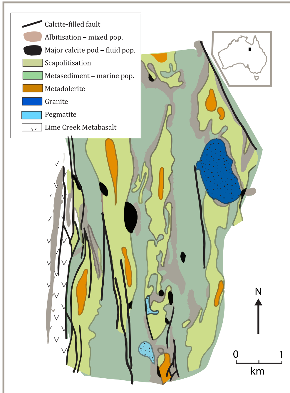
Figure 4.7. Geologic-alteration map of part of the Mary Kathleen Fold Belt, about 9 km NNE of MK, with carbonate \delta^{18}\text{O} – \delta^{13}\text{C} populations (from Oliver & Wall, 1987, modified).
