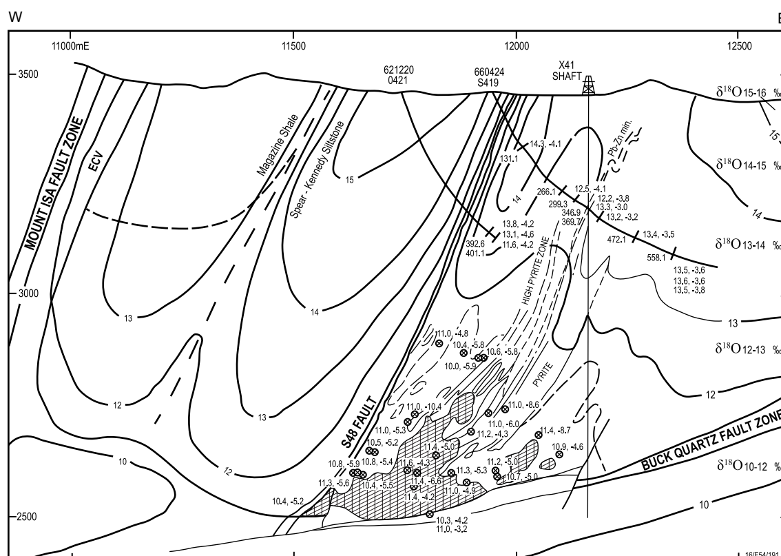
Figure 4.1. Composite cross section of Mount Isa Mine centred at 34200 mN showing carbonate O and C isotopic data along drill holes, interpreted \delta^{18}\text{O} contours and the simplified geology (from Waring et al. , 1998).
