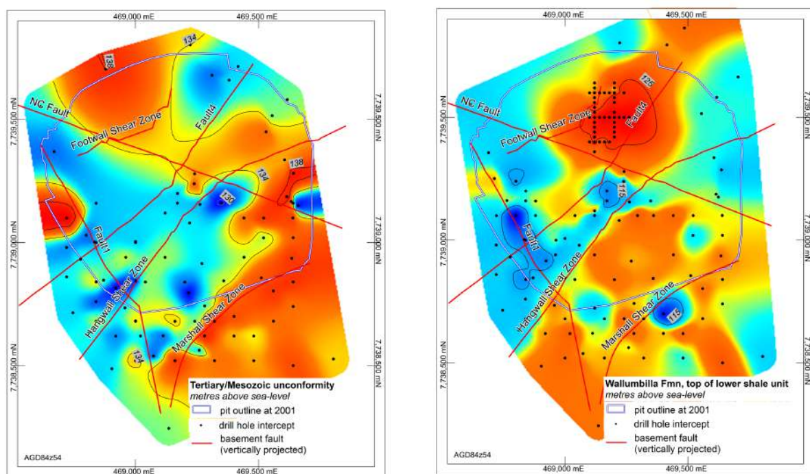
Figure 6.4. Relationship of major structures to the gridded intercepts of two paleosurfaces: left frame—Tertiary unconformity, right frame—top of the lower shale unit of the Wallumbilla Formation (modifications of figures 16 and 18 of Sheppard, 2001). The pre-mining surface RL was about 156 m (ASL).
